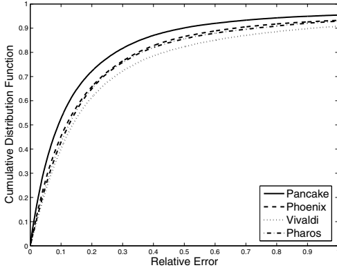
(a) PlanetLab
