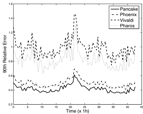
Fig. 7. Relative Error for the “K200-allpairs-1h” Data Set
