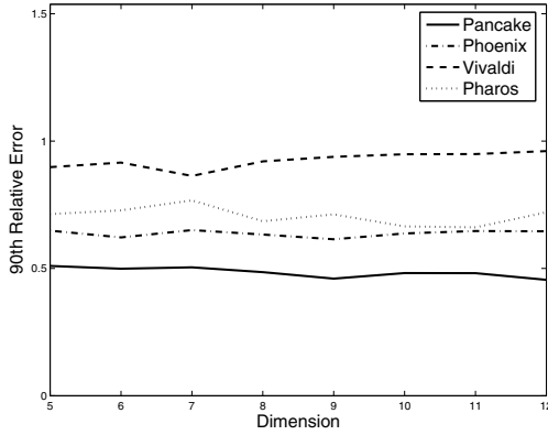
(a) PlanetLab
