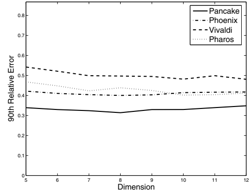
(b) King
