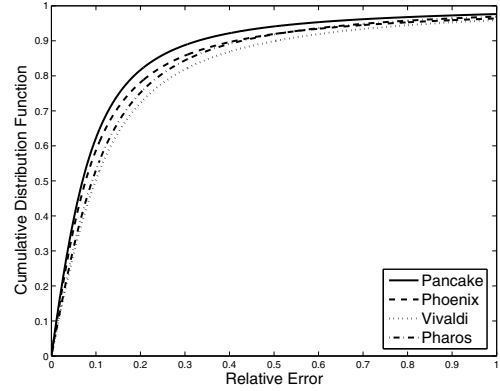
(b) King
