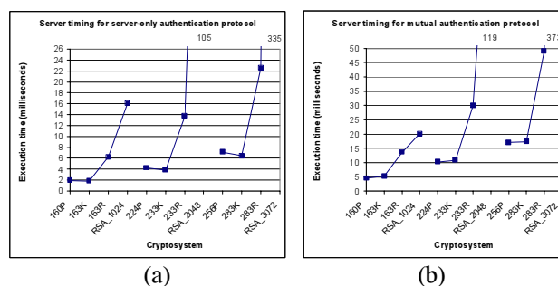
Figure 5. Server's processing time of public-key cryptosystem operations (a) in the handshake protocol with server-only authentication (protocol 1), (b) in the handshake protocol with mutual authentication (protocol 2)
